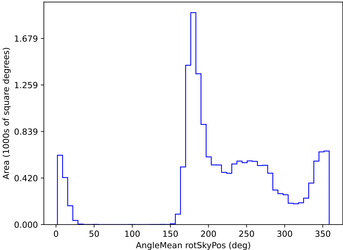
too_elab_r8_d2_gz_v3.4_10yrs WFD y band: AngleMean rotSkyPos
