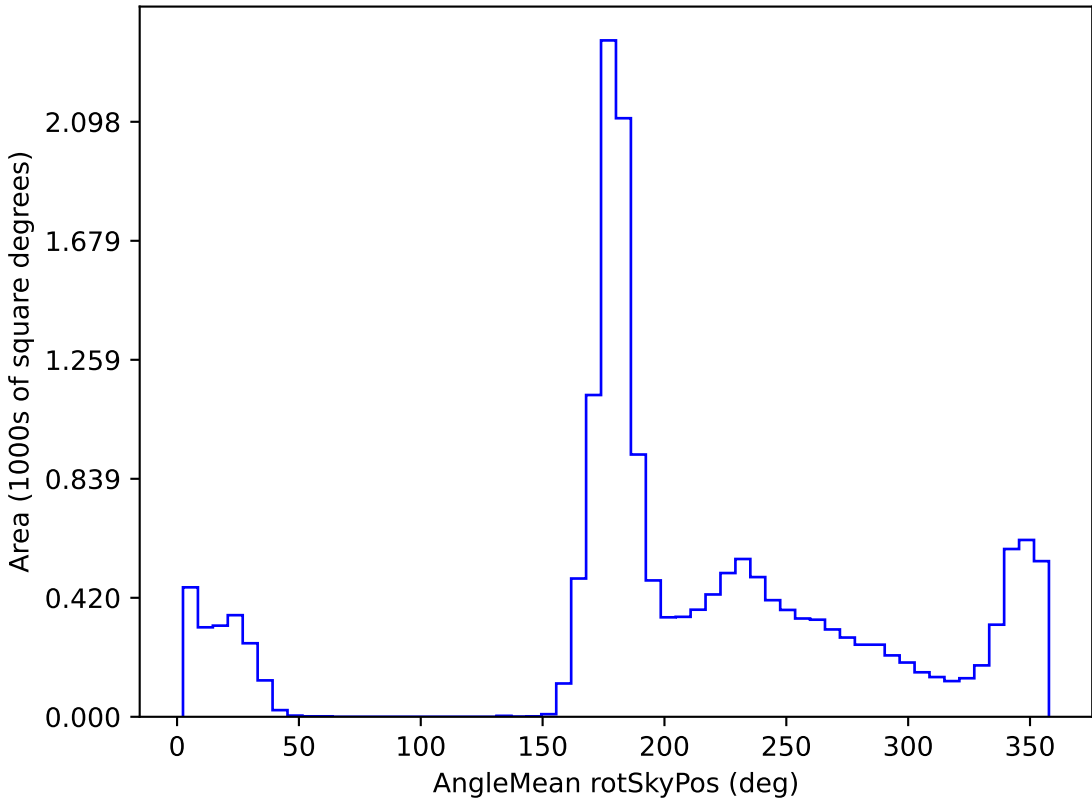
too_elab_r8_d2_gz_v3.4_10yrs WFD r band: AngleMean rotSkyPos
