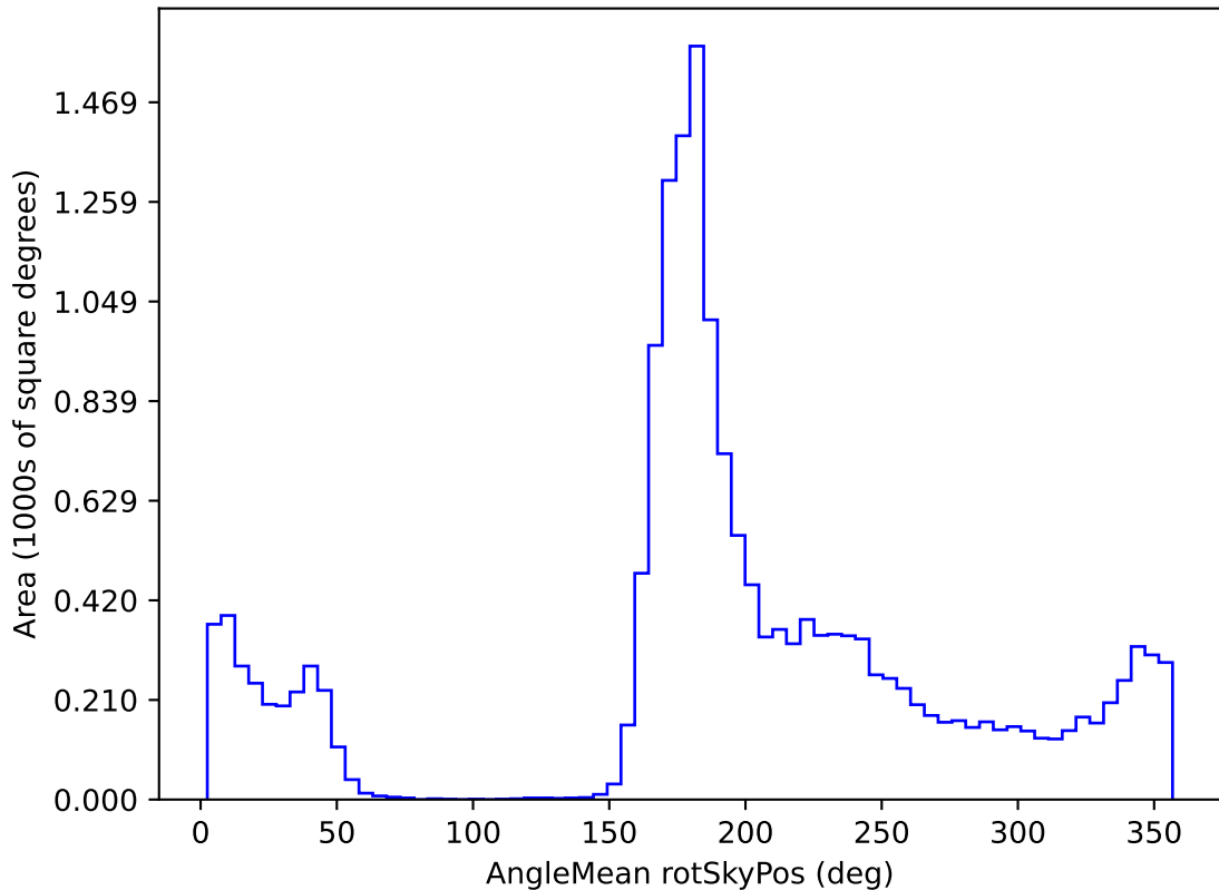
too_elab_r8_d2_gz_v3.4_10yrs WFD g band: AngleMean rotSkyPos
