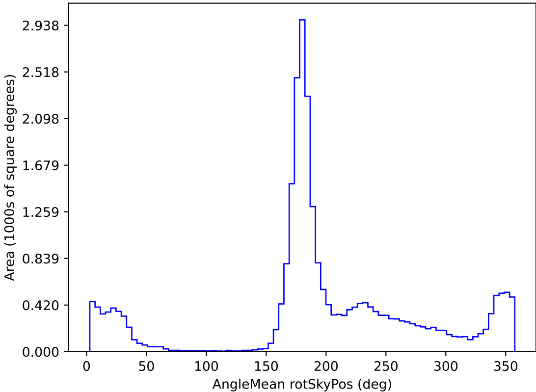
too_elab_r8_d2_gz_v3.4_10yrs All sky r band: AngleMean rotSkyPos
