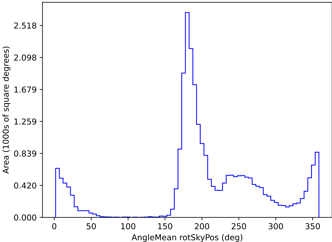
too_elab_r8_d2_gz_v3.4_10yrs All sky i band: AngleMean rotSkyPos
