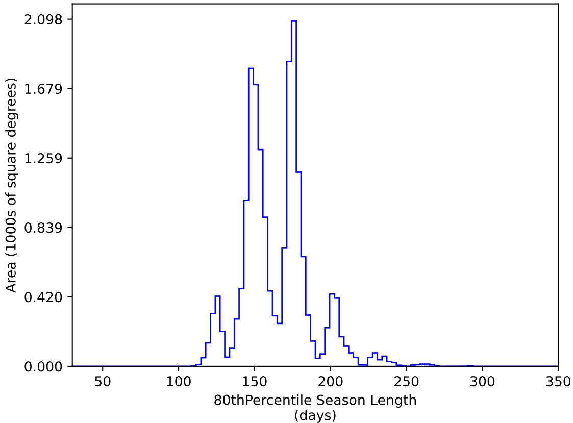
too_elab_r8_d2_gz_v3.4_10yrs WFD y band: 80thPercentile Season Length
