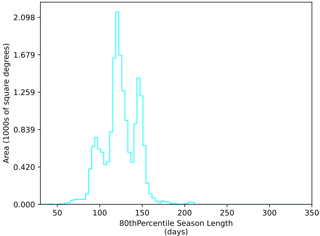
too_elab_r8_d2_gz_v3.4_10yrs WFD u band: 80thPercentile Season Length
