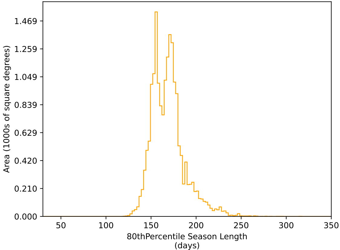
too_elab_r8_d2_gz_v3.4_10yrs WFD r band: 80thPercentile Season Length
