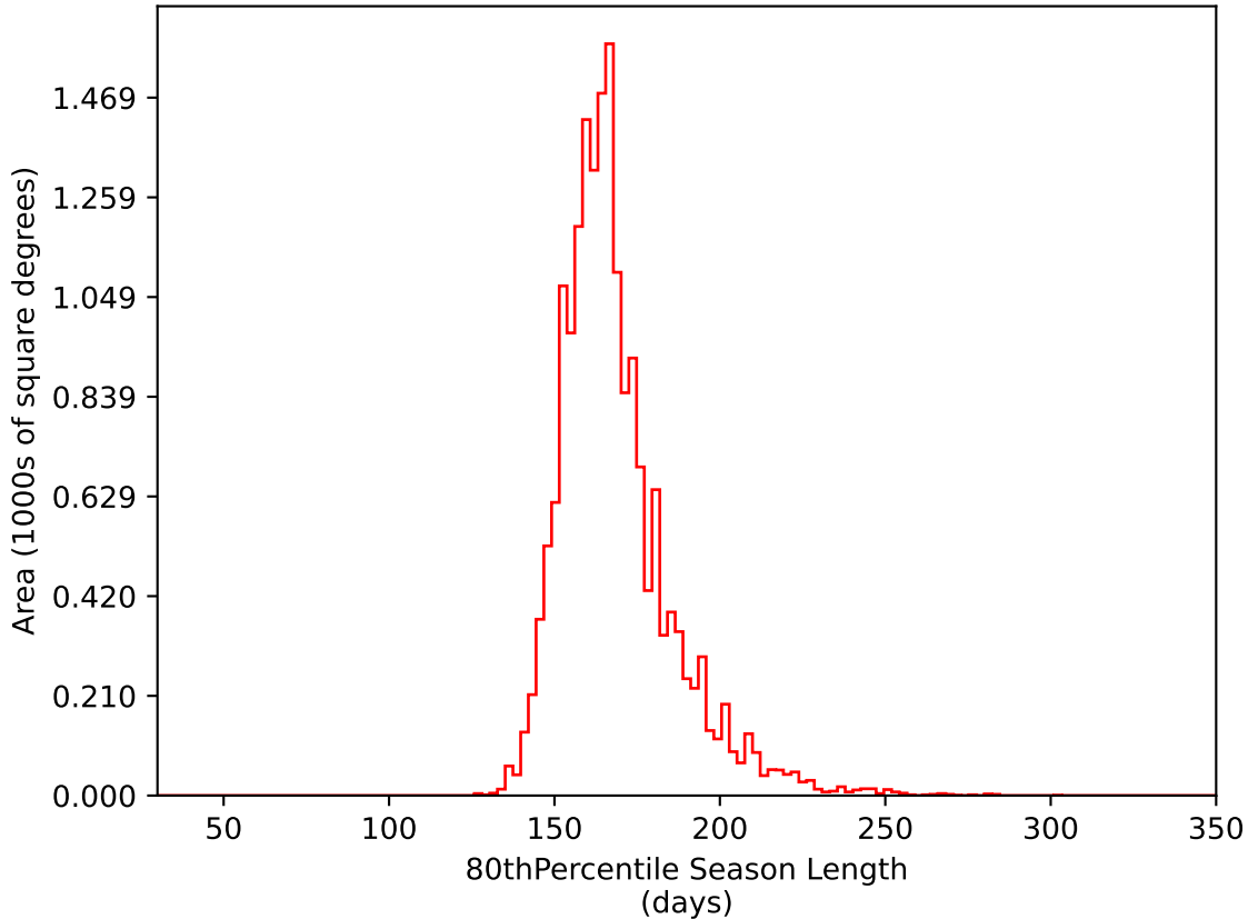
too_elab_r8_d2_gz_v3.4_10yrs WFD i band: 80thPercentile Season Length
