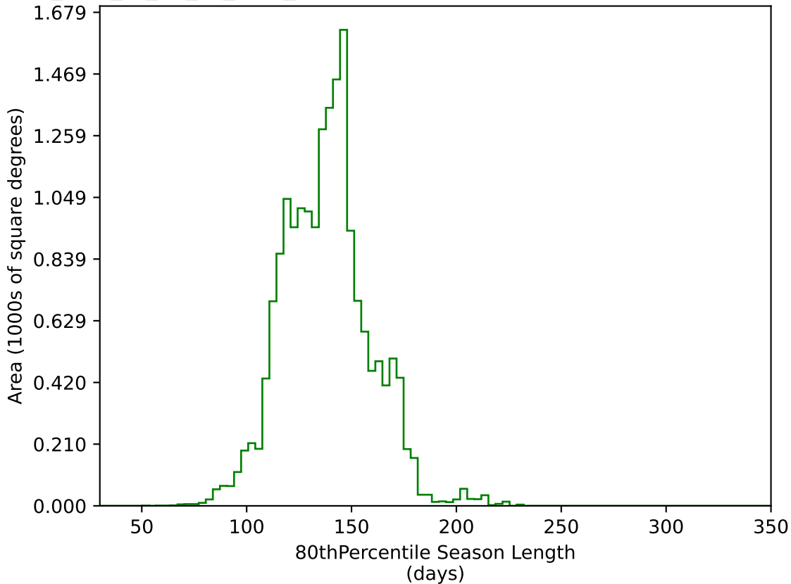
too_elab_r8_d2_gz_v3.4_10yrs WFD g band: 80thPercentile Season Length
