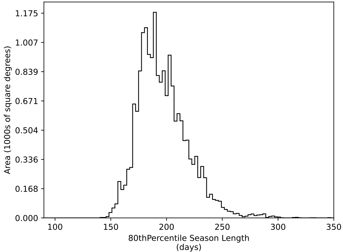
too_elab_r8_d2_gz_v3.4_10yrs WFD all bands: 80thPercentile Season Length
