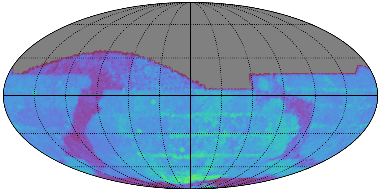
too_elab_r8_d2_gz_v3.4_10yrs All sky z band: 80thPercentile Season Length
