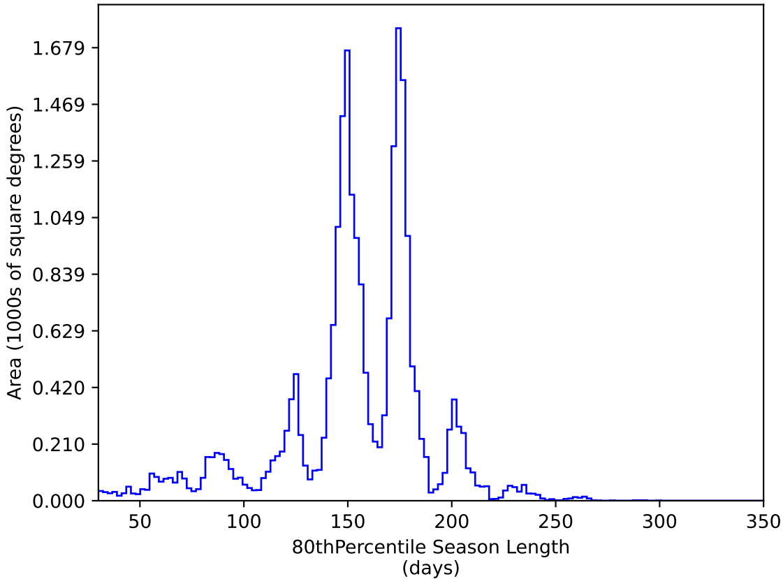
too_elab_r8_d2_gz_v3.4_10yrs All sky y band: 80thPercentile Season Length
