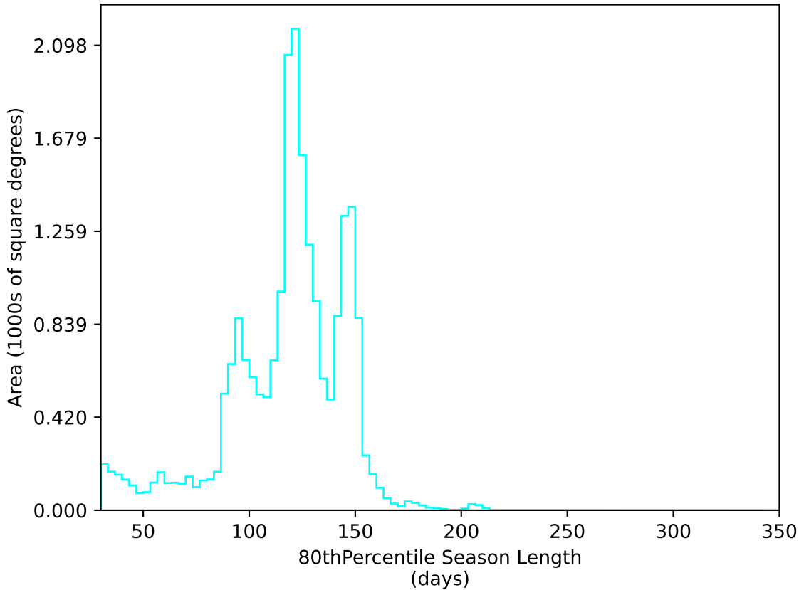
too_elab_r8_d2_gz_v3.4_10yrs All sky u band: 80thPercentile Season Length
