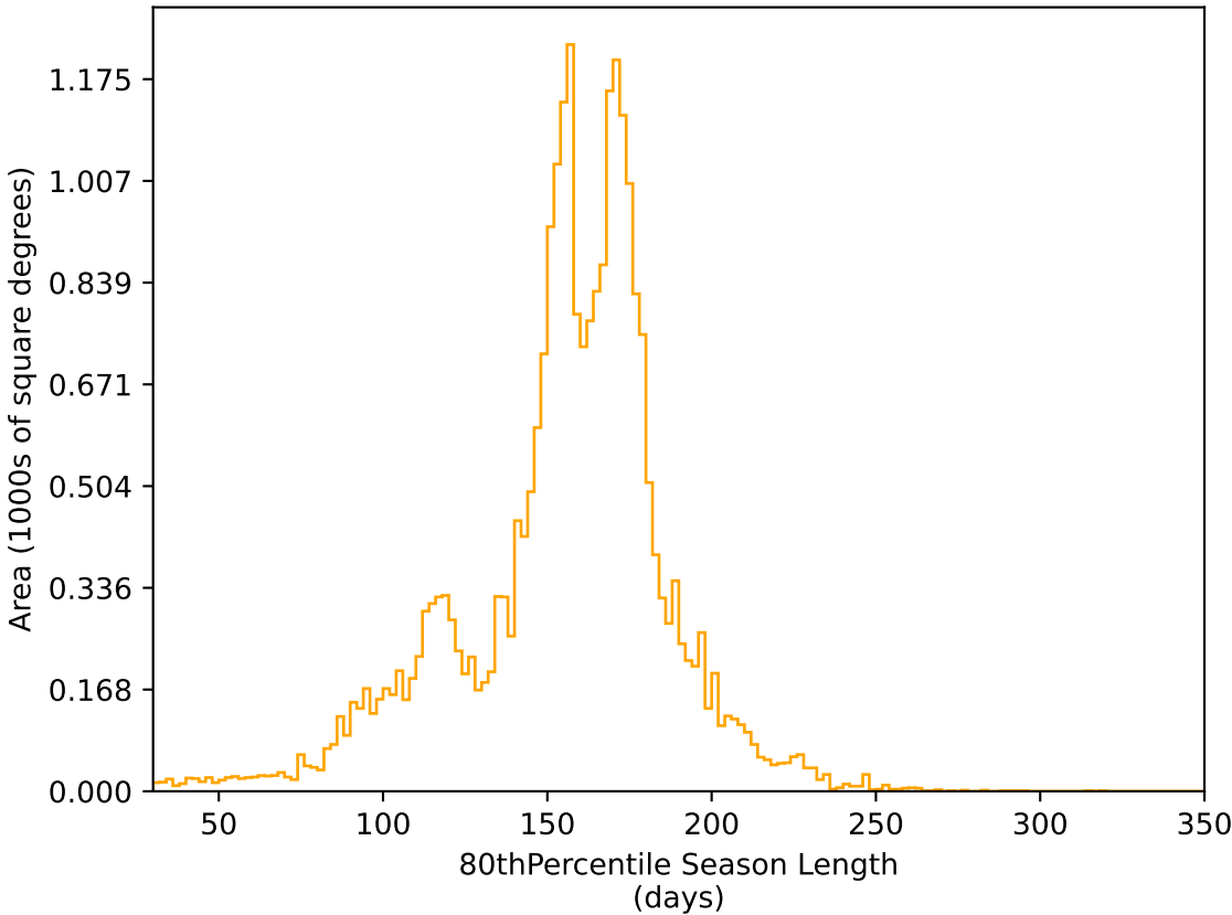
too_elab_r8_d2_gz_v3.4_10yrs All sky r band: 80thPercentile Season Length
