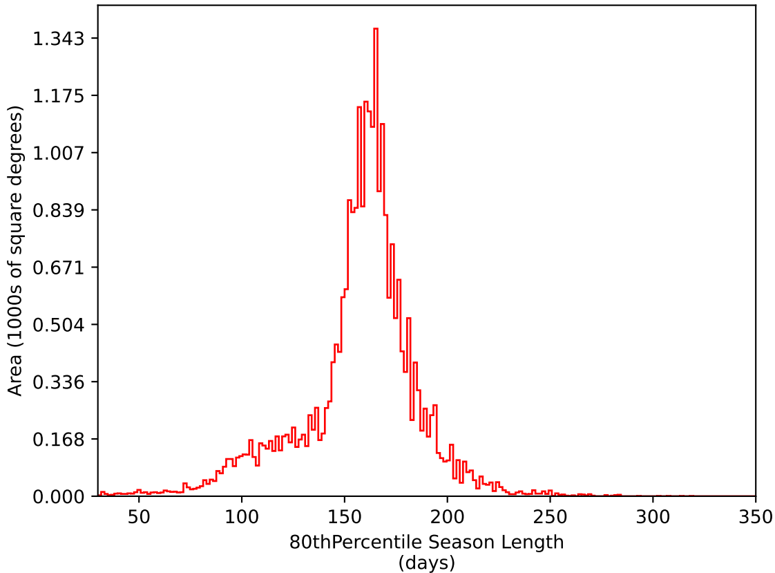
too_elab_r8_d2_gz_v3.4_10yrs All sky i band: 80thPercentile Season Length
