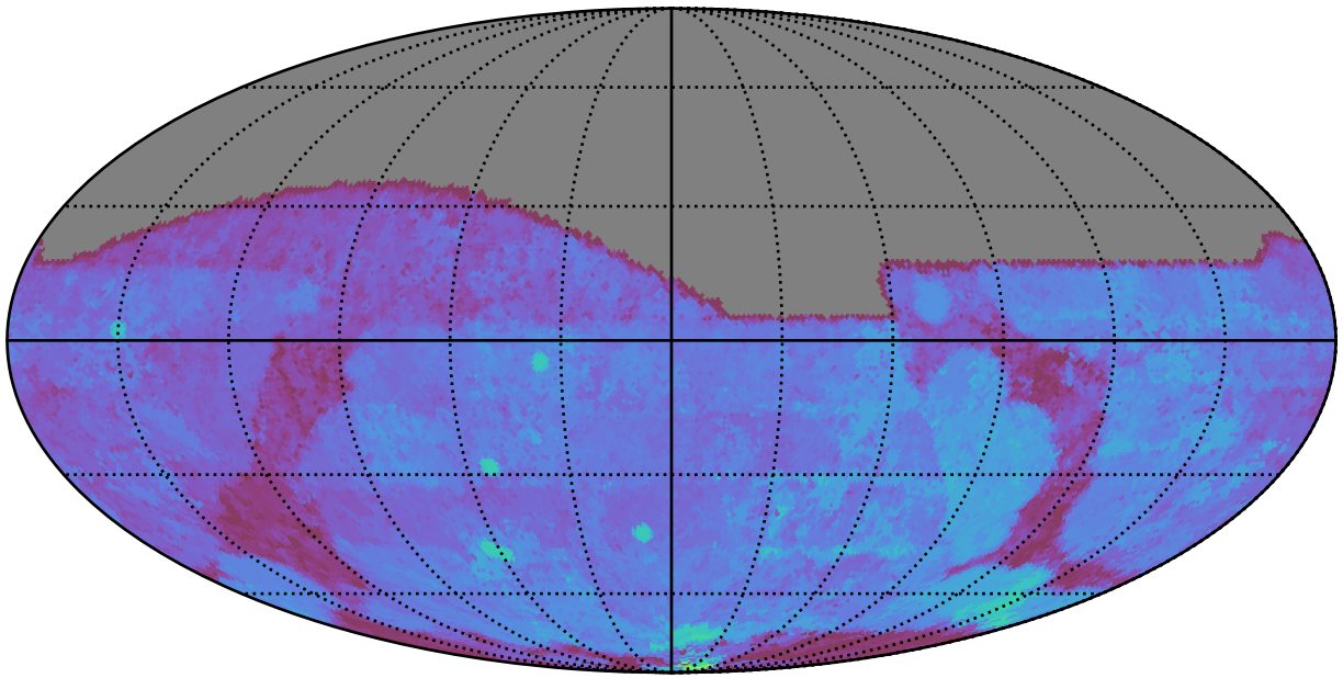
too_elab_r8_d2_gz_v3.4_10yrs All sky g band: 80thPercentile Season Length
