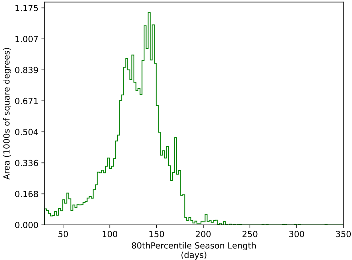
too_elab_r8_d2_gz_v3.4_10yrs All sky g band: 80thPercentile Season Length
