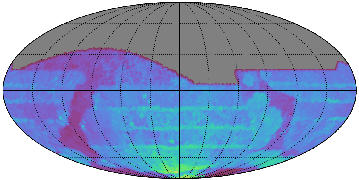
too_elab_r8_d2_gz_v3.4_10yrs All sky all bands: 80thPercentile Season Length
