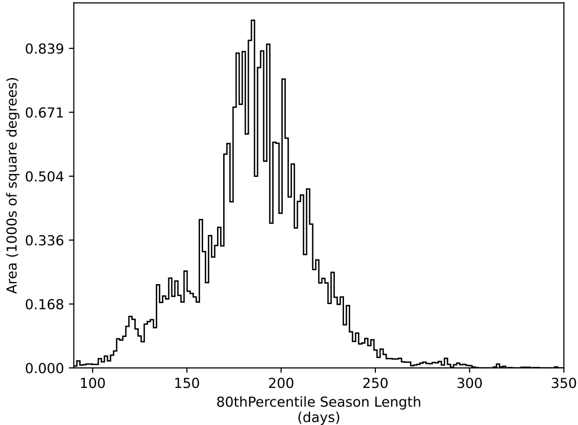
too_elab_r8_d2_gz_v3.4_10yrs All sky all bands: 80thPercentile Season Length
