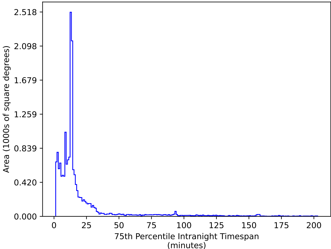
too_elab_r8_d2_gz_v3.4_10yrs WFD z band: 75th Percentile Intranight Timespan
