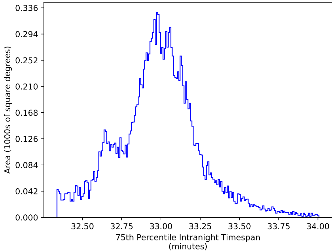
too_elab_r8_d2_gz_v3.4_10yrs WFD y band: 75th Percentile Intranight Timespan
