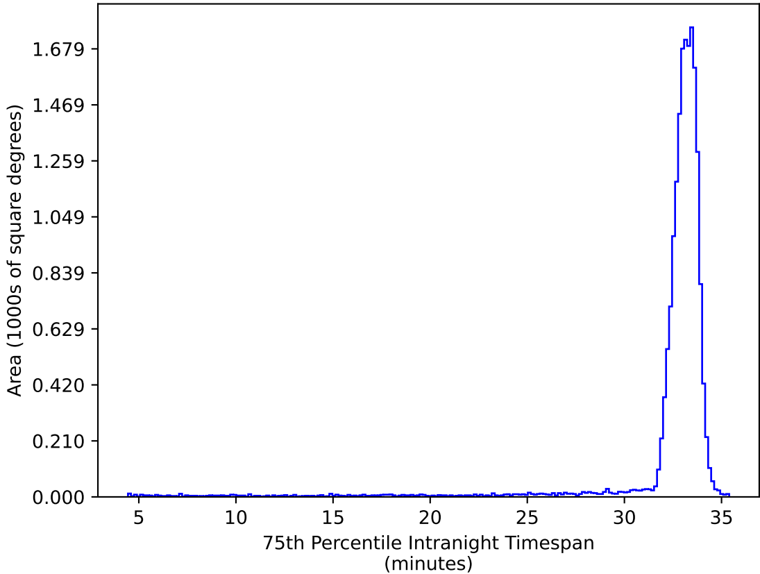
too_elab_r8_d2_gz_v3.4_10yrs WFD ug bands: 75th Percentile Intranight Timespan
