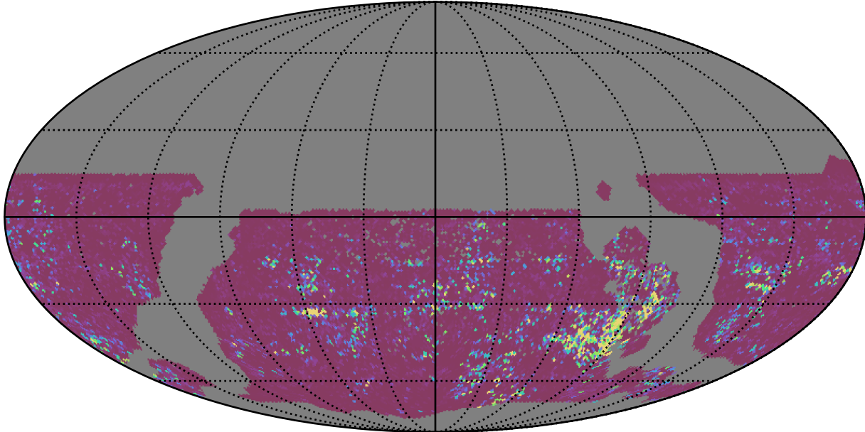
too_elab_r8_d2_gz_v3.4_10yrs WFD u band: 75th Percentile Intranight Timespan
