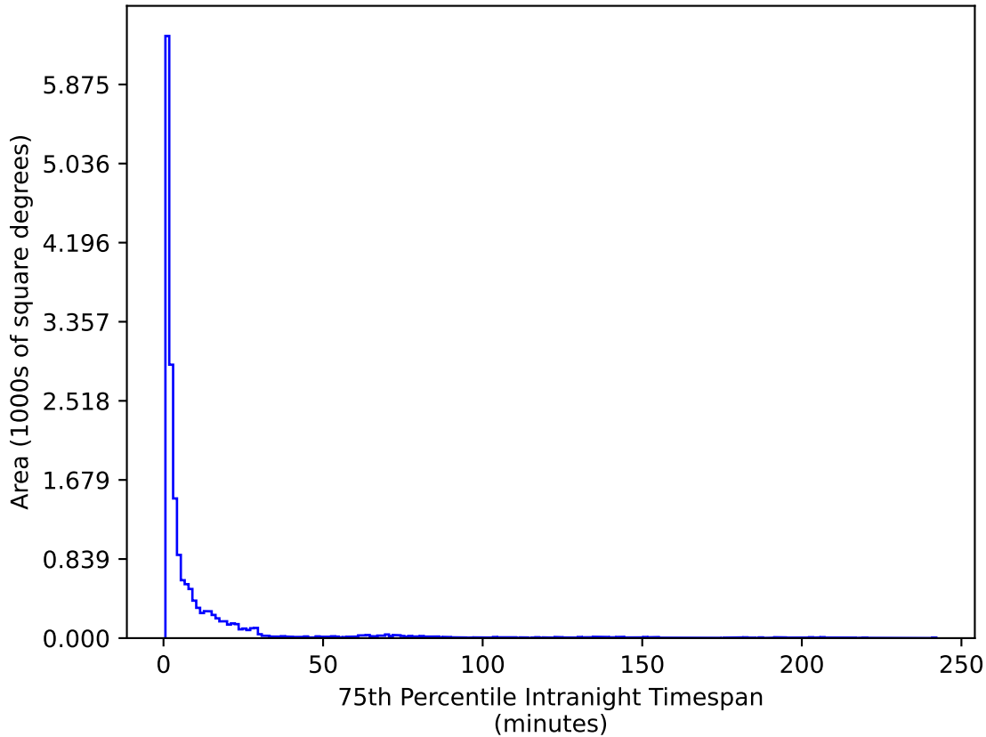
too_elab_r8_d2_gz_v3.4_10yrs WFD u band: 75th Percentile Intranight Timespan
