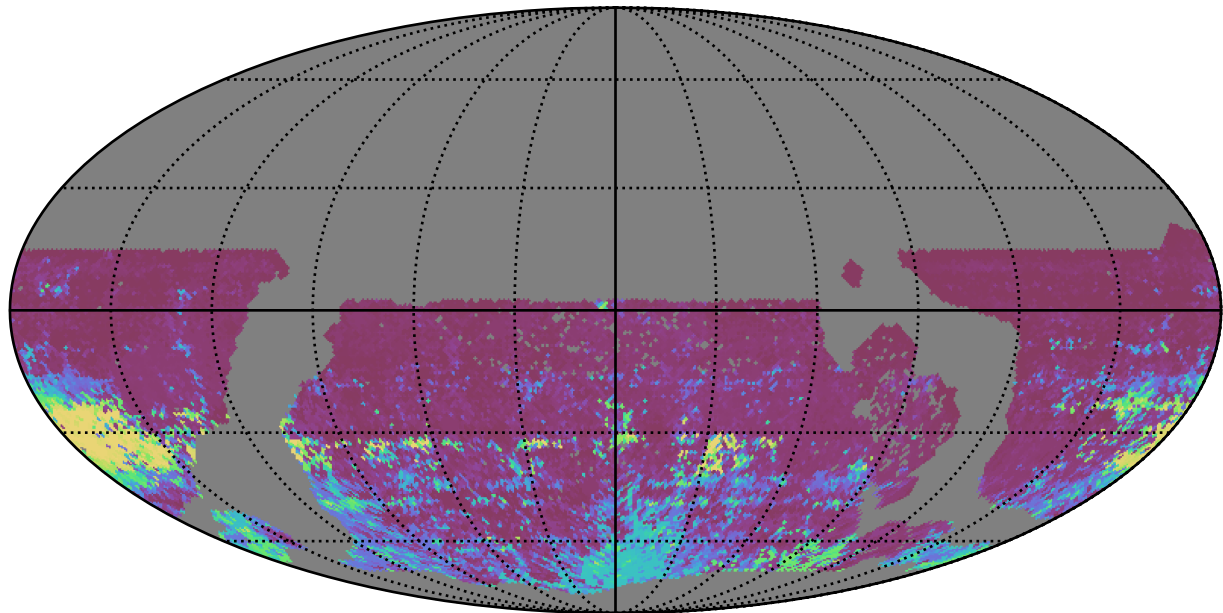
too_elab_r8_d2_gz_v3.4_10yrs WFD r band: 75th Percentile Intranight Timespan
