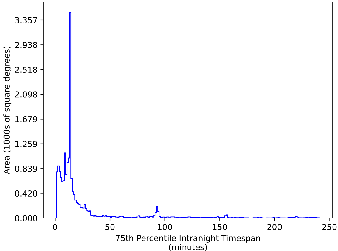
too_elab_r8_d2_gz_v3.4_10yrs WFD i band: 75th Percentile Intranight Timespan
