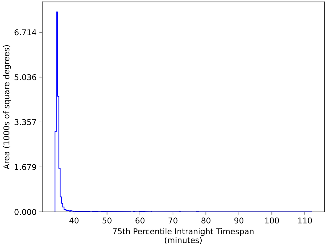
too_elab_r8_d2_gz_v3.4_10yrs WFD gr bands: 75th Percentile Intranight Timespan
