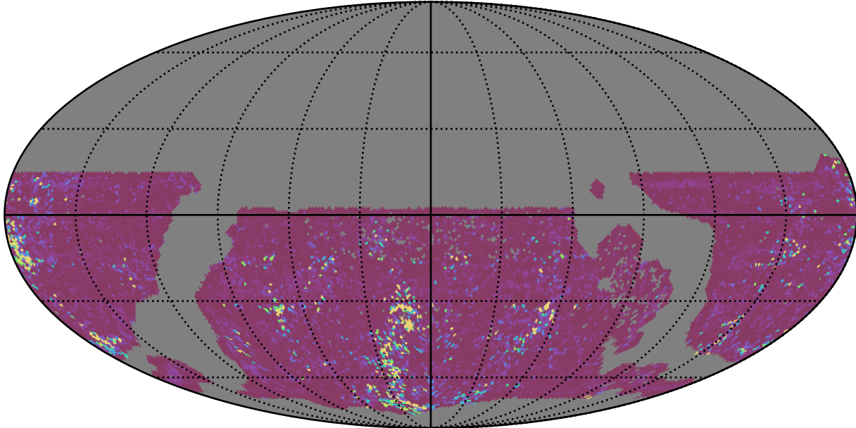
too_elab_r8_d2_gz_v3.4_10yrs WFD g band: 75th Percentile Intranight Timespan
