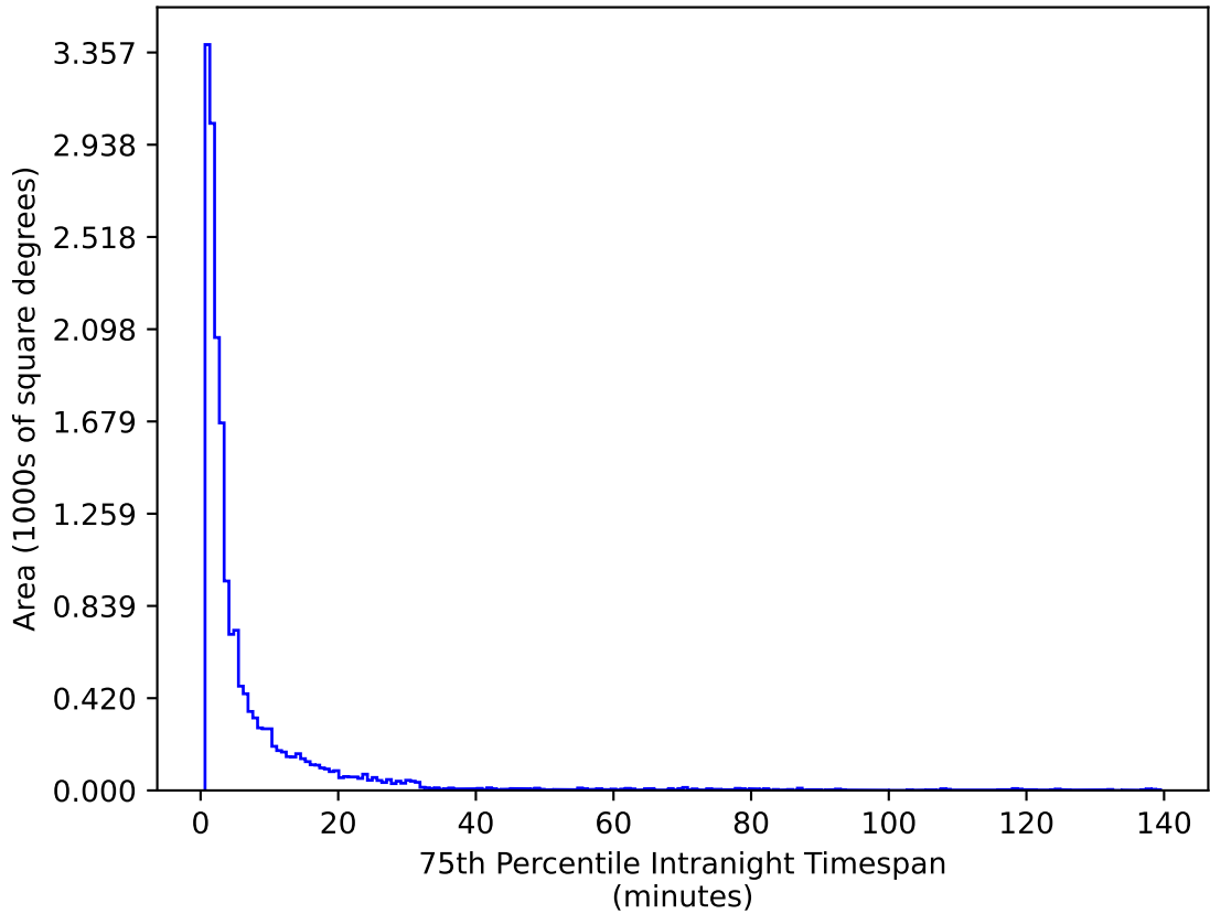
too_elab_r8_d2_gz_v3.4_10yrs WFD g band: 75th Percentile Intranight Timespan
