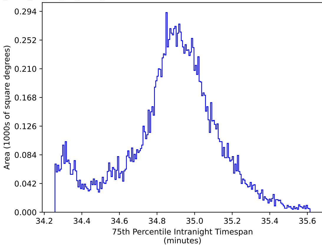
too_elab_r8_d2_gz_v3.4_10yrs WFD all bands: 75th Percentile Intranight Timespan
