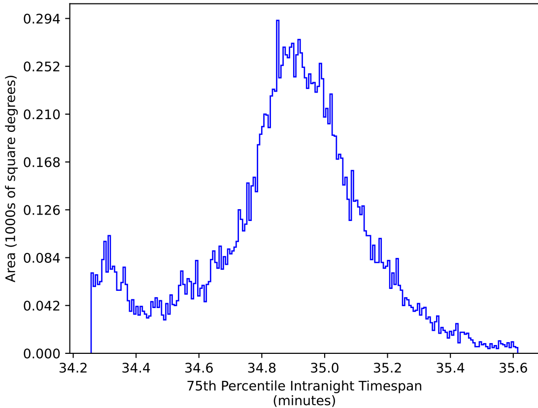
too_elab_r8_d2_gz_v3.4_10yrs WFD: 75th Percentile Intranight Timespan
