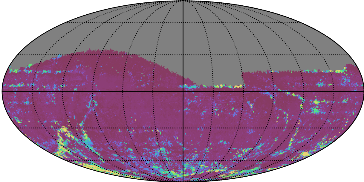
too_elab_r8_d2_gz_v3.4_10yrs All sky z band: 75th Percentile Intranight Timespan
