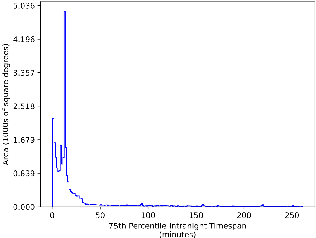
too_elab_r8_d2_gz_v3.4_10yrs All sky z band: 75th Percentile Intranight Timespan
