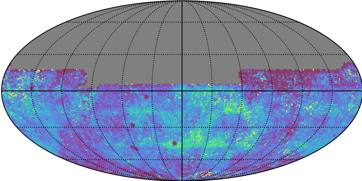
too_elab_r8_d2_gz_v3.4_10yrs All sky y band: 75th Percentile Intranight Timespan
