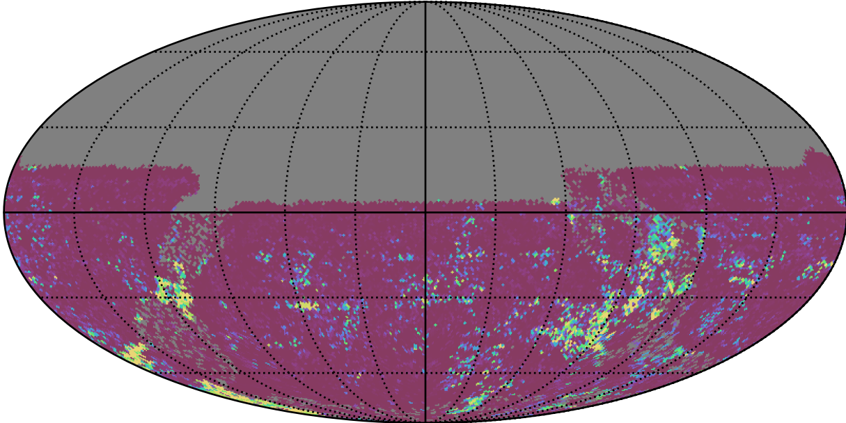
too_elab_r8_d2_gz_v3.4_10yrs All sky u band: 75th Percentile Intranight Timespan
