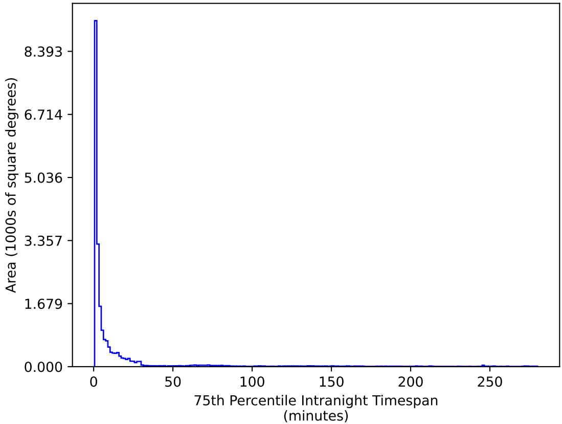
too_elab_r8_d2_gz_v3.4_10yrs All sky u band: 75th Percentile Intranight Timespan
