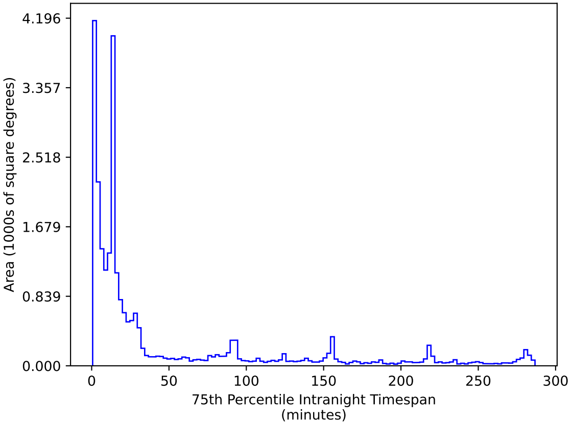
too_elab_r8_d2_gz_v3.4_10yrs All sky r band: 75th Percentile Intranight Timespan
