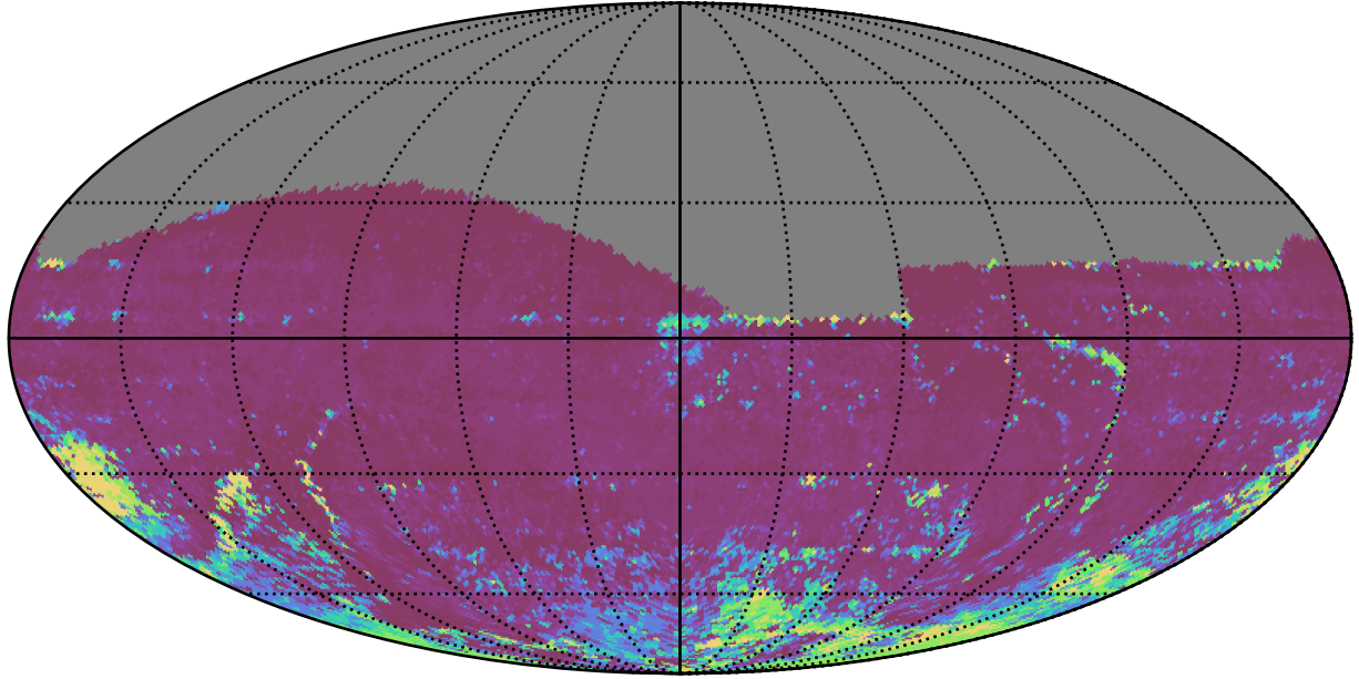
too_elab_r8_d2_gz_v3.4_10yrs All sky i band: 75th Percentile Intranight Timespan
