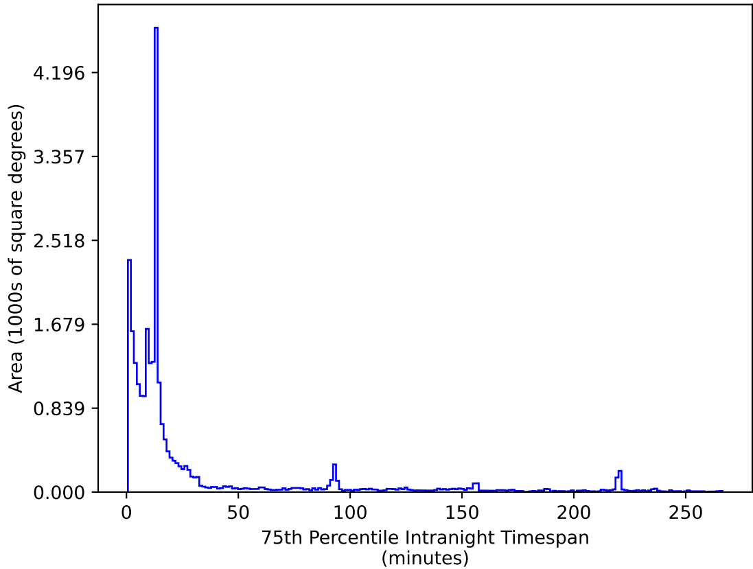
too_elab_r8_d2_gz_v3.4_10yrs All sky i band: 75th Percentile Intranight Timespan
