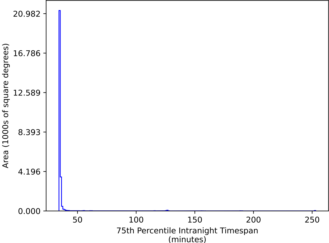
too_elab_r8_d2_gz_v3.4_10yrs All sky gr bands: 75th Percentile Intranight Timespan
