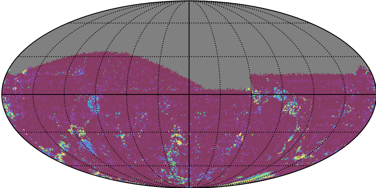
too_elab_r8_d2_gz_v3.4_10yrs All sky g band: 75th Percentile Intranight Timespan
