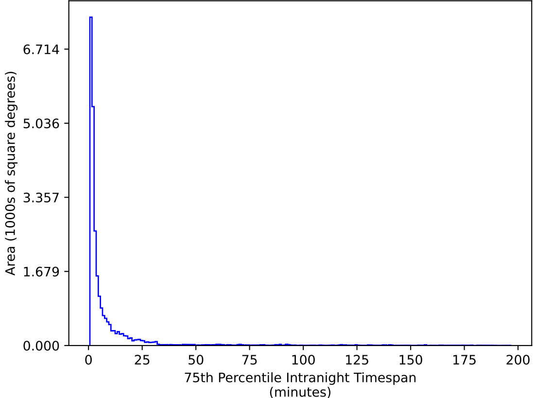
too_elab_r8_d2_gz_v3.4_10yrs All sky g band: 75th Percentile Intranight Timespan
