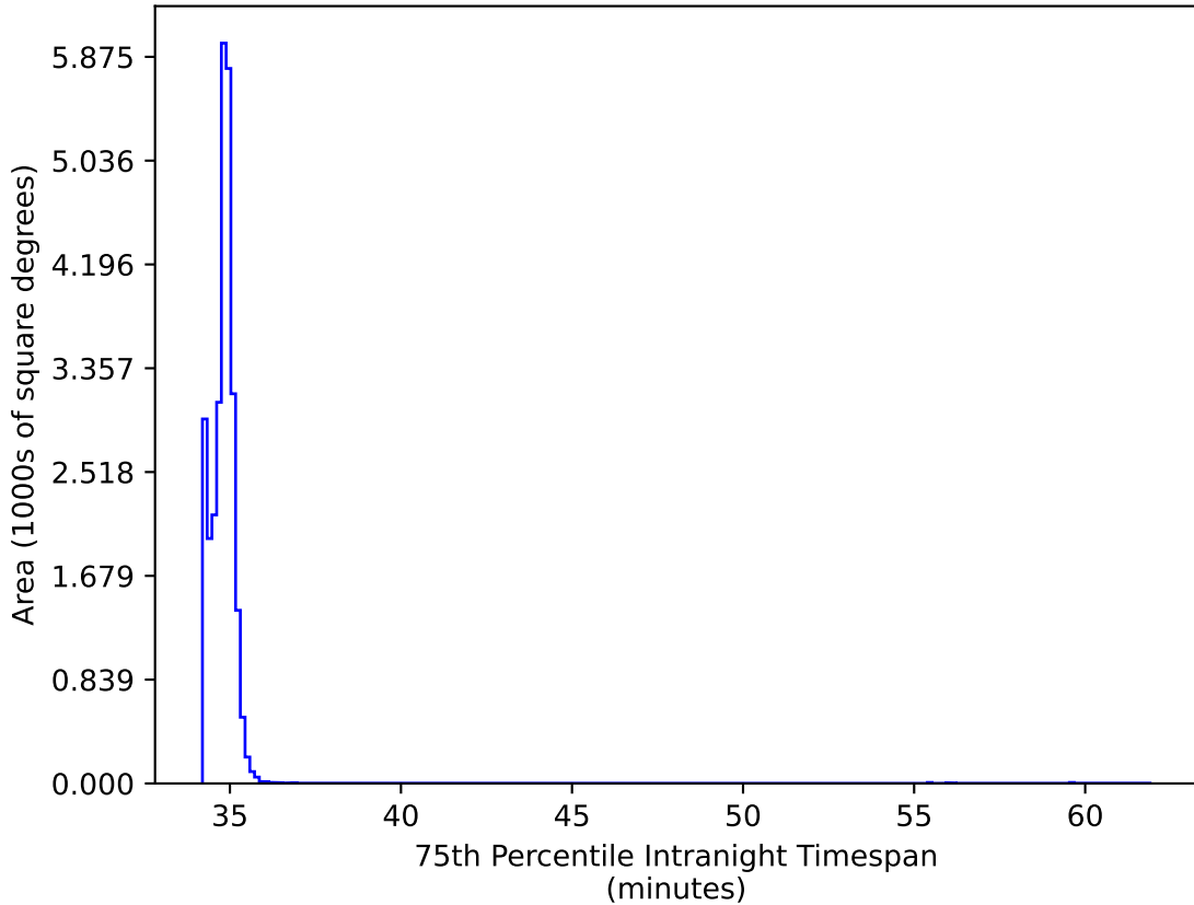
too_elab_r8_d2_gz_v3.4_10yrs All sky: 75th Percentile Intranight Timespan
