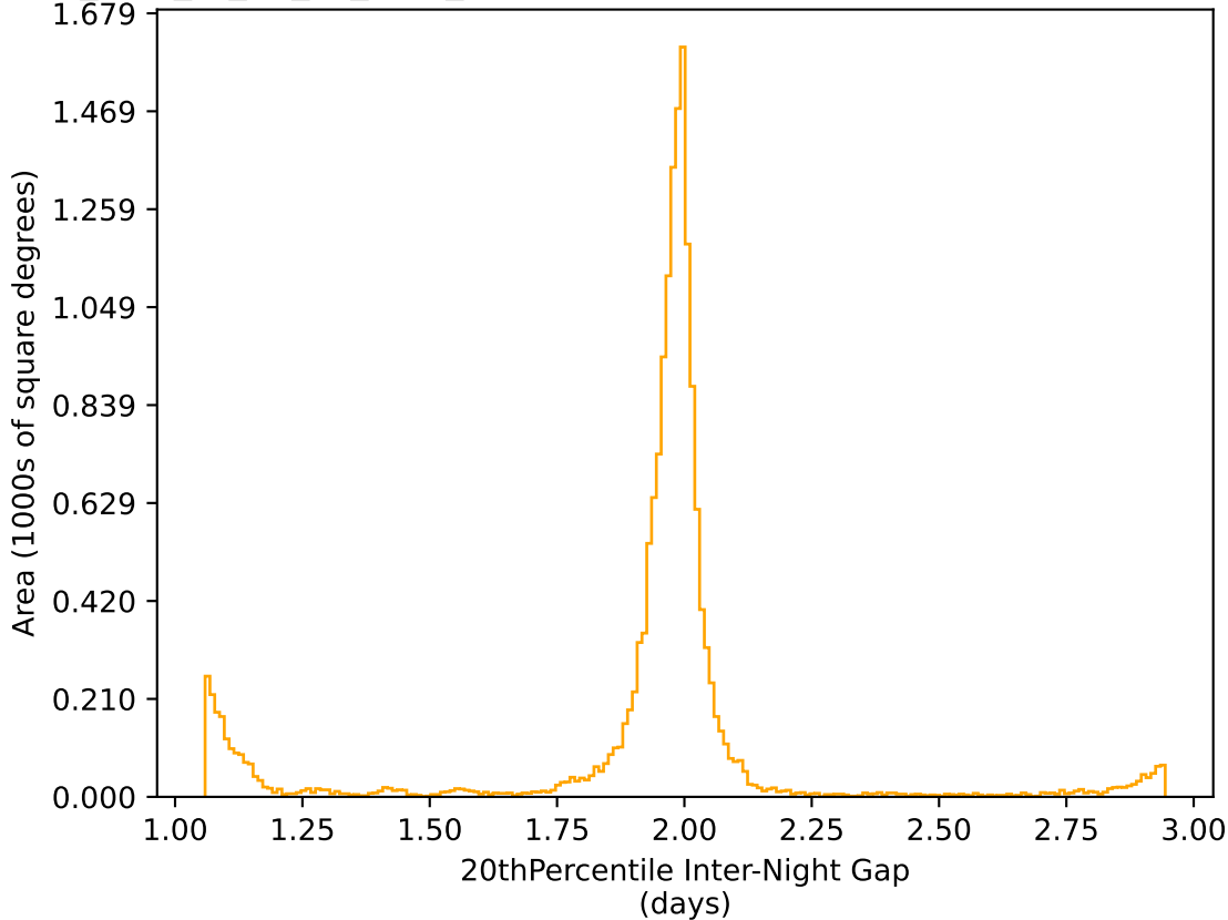
too_elab_r8_d2_gz_v3.4_10yrs WFD r band: 20thPercentile Inter-Night Gap
