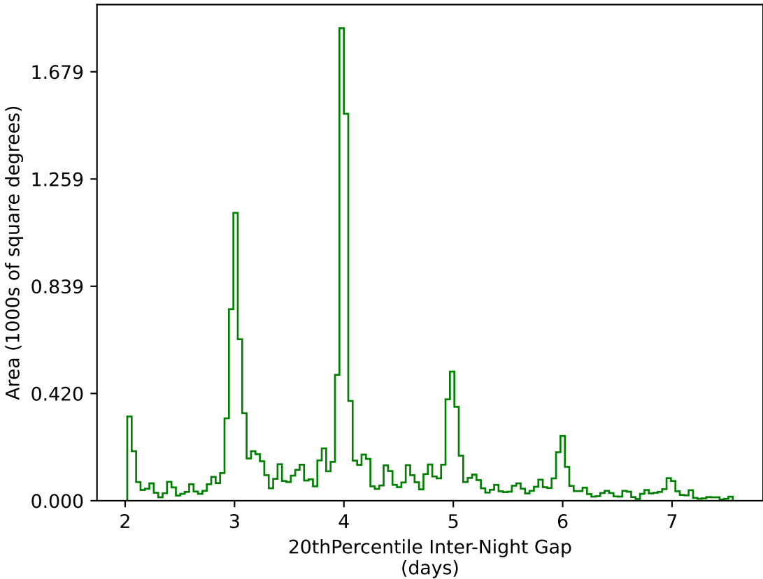
too_elab_r8_d2_gz_v3.4_10yrs WFD g band: 20thPercentile Inter-Night Gap
