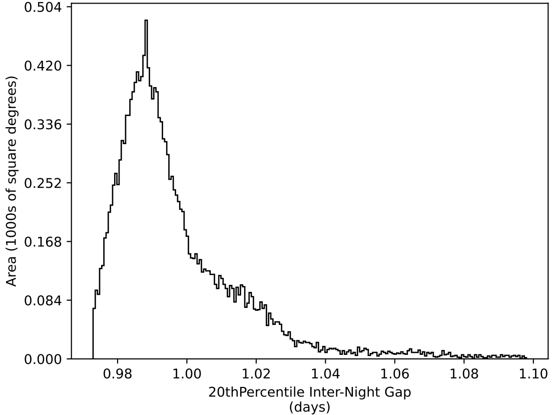
too_elab_r8_d2_gz_v3.4_10yrs WFD all bands: 20thPercentile Inter-Night Gap
