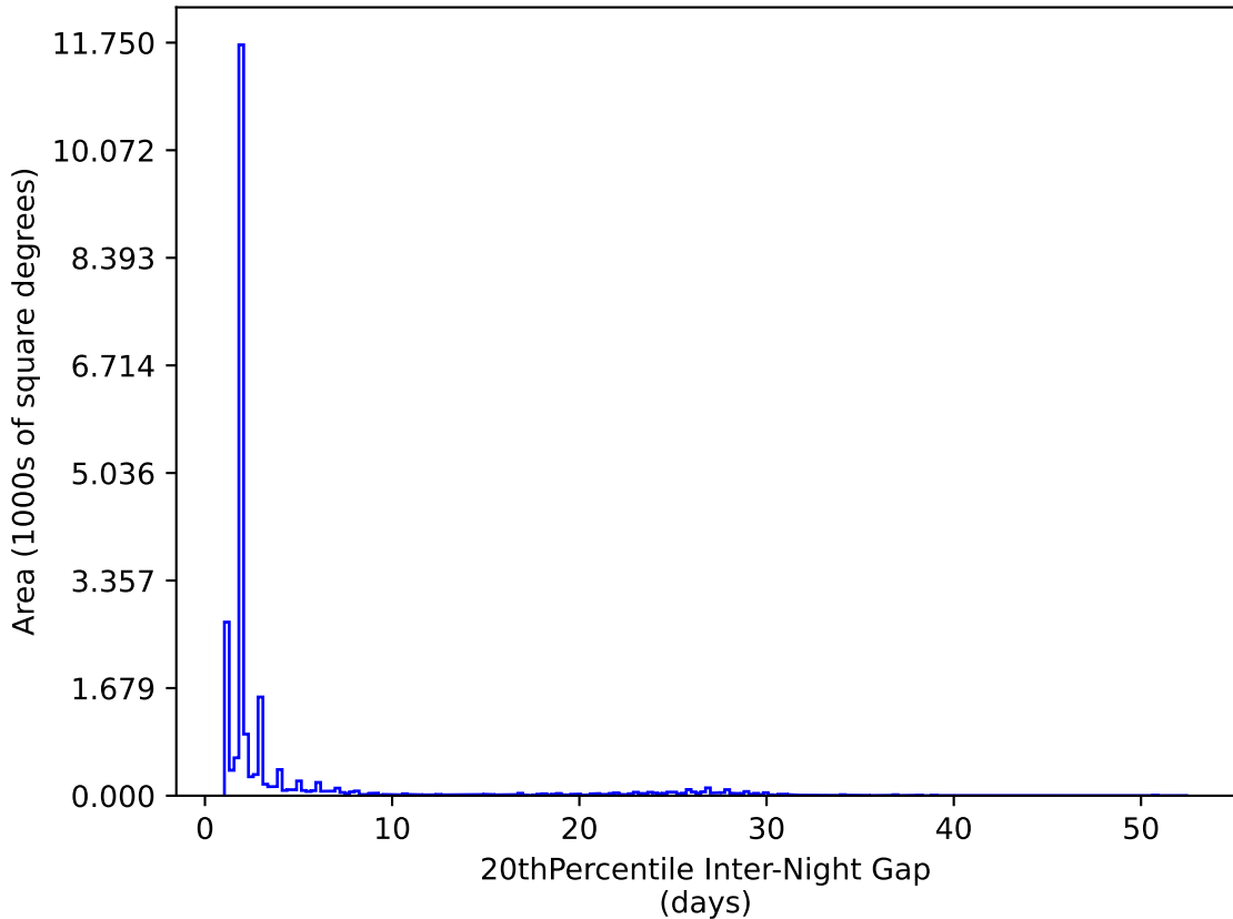
too_elab_r8_d2_gz_v3.4_10yrs All sky y band: 20thPercentile Inter-Night Gap
