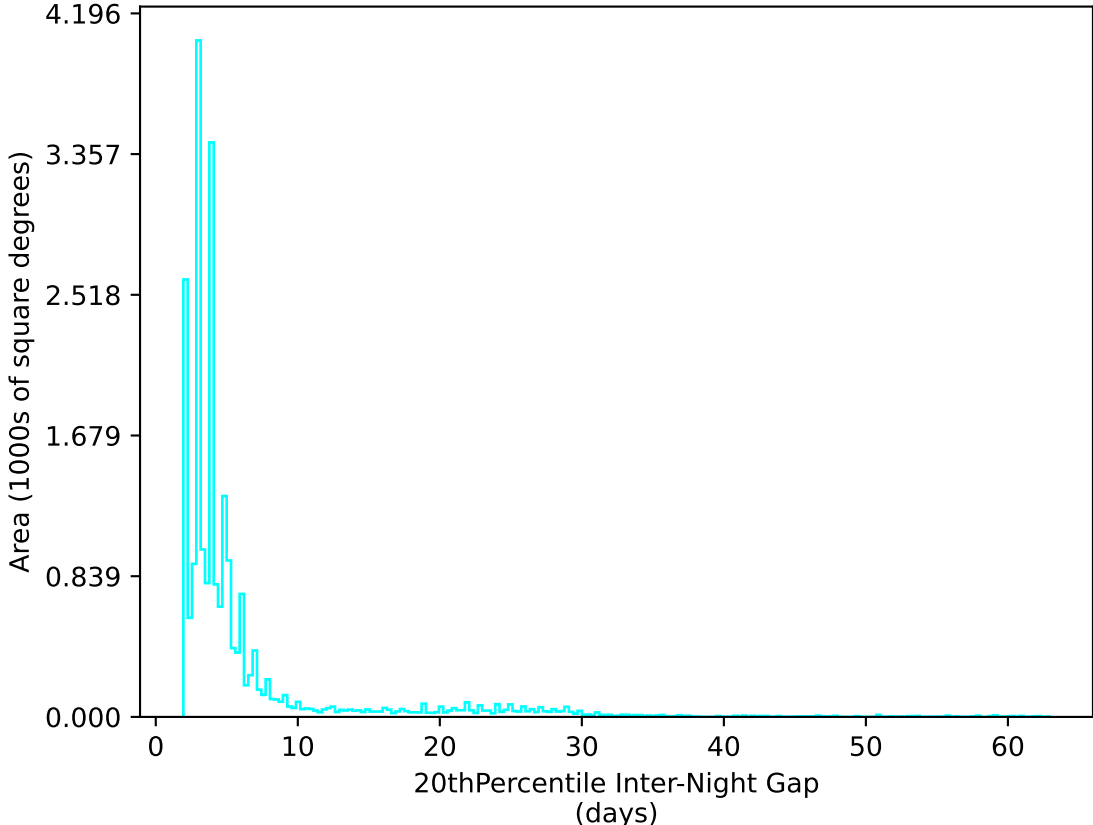
too_elab_r8_d2_gz_v3.4_10yrs All sky u band: 20thPercentile Inter-Night Gap
