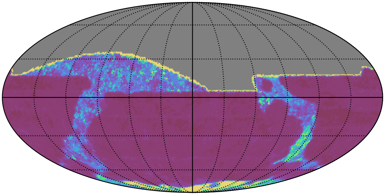
too_elab_r8_d2_gz_v3.4_10yrs All sky r band: 20thPercentile Inter-Night Gap
